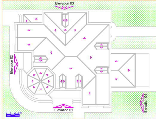
Roof Plan
