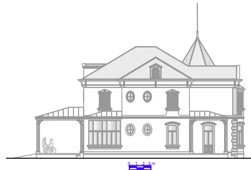
Elevation 03
